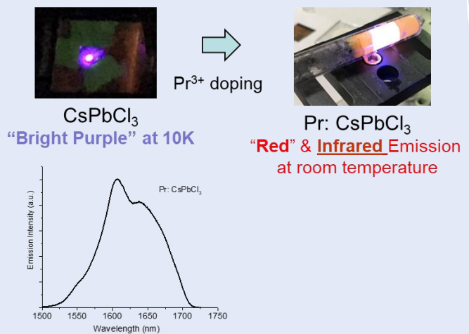
Increased emission coverage of CsPbCl 3 through rare earth doping.
